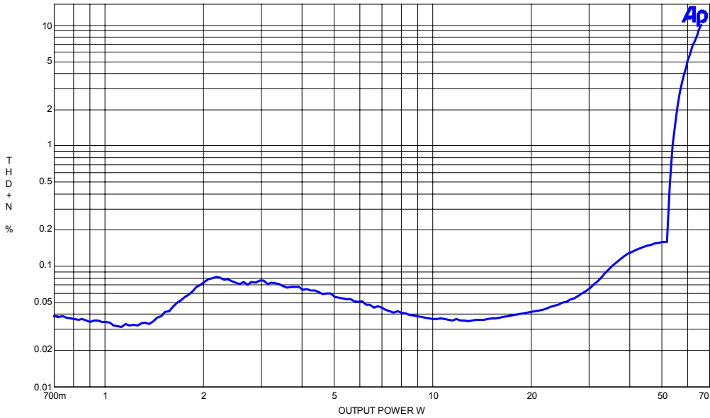
Figure 1. THD+N vs Power
