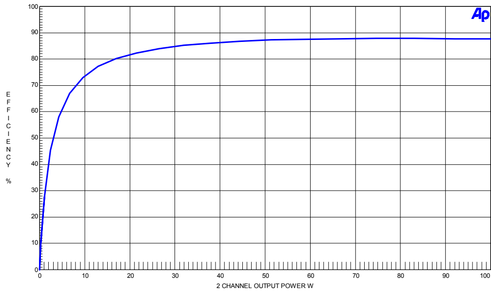
Figure 8. Output Stage Efficiency
