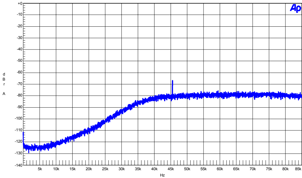
Figure 4. Noise Floor
