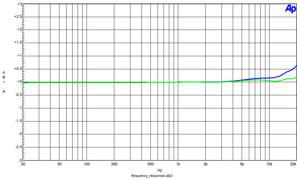
Figure 6. Frequency Response
