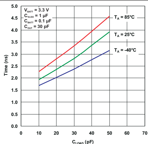
Figure 7-9. Fall Time vs Load
