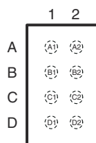
Figure 6-1. YFP Package 8-Pin DSBGA Top View
