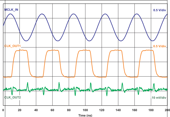
Figure 7-10. Digital Cross-Talk Scope Shot
