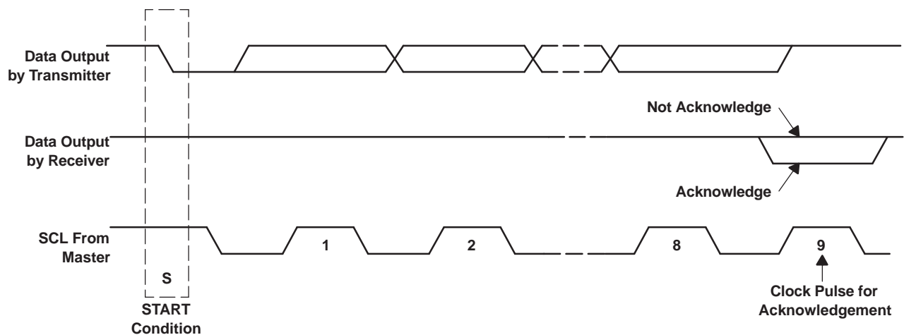
Figure 52. Acknowledge on the I²C Bus
