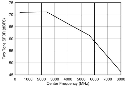
Figure 5-109. Dual Channel Mode: Two Tone SFDR vs Input Frequency
