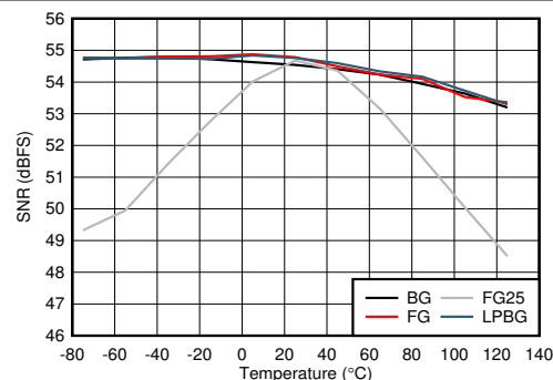
Figure 5-92. Dual Channel Mode: SNR vs Temperature and Calibration Mode
