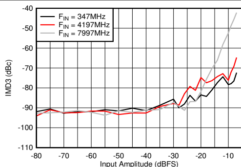
Figure 5-107. Dual Channel Mode: IMD3 vs Input Amplitude
