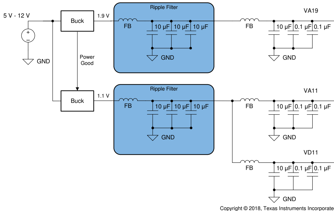
Figure 7-6. Switcher-Only Approach Example
