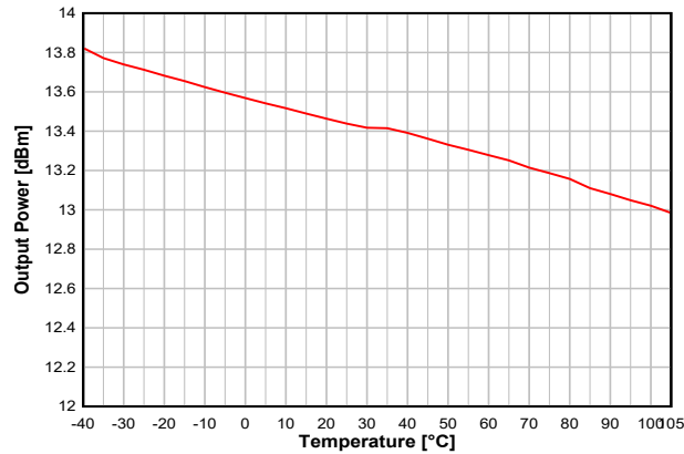
Figure 8-18. Output Power vs. Temperature (50 kbps, 868.3 MHz)
