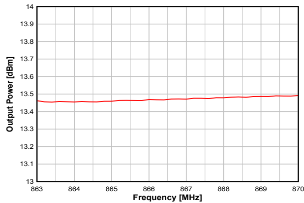
Figure 8-20. Output Power vs. Frequency (50 kbps, 868 MHz)
