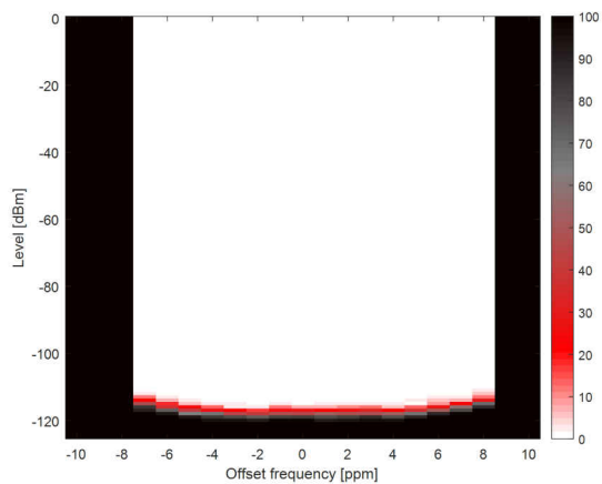
Figure 8-17. PER vs. Level vs. Frequency (Narrowband, 9.6 kbps, \pm 2.4 kHz deviation, 2-GFSK, 868 MHz, 17.1 kHz RX bandwidth)
