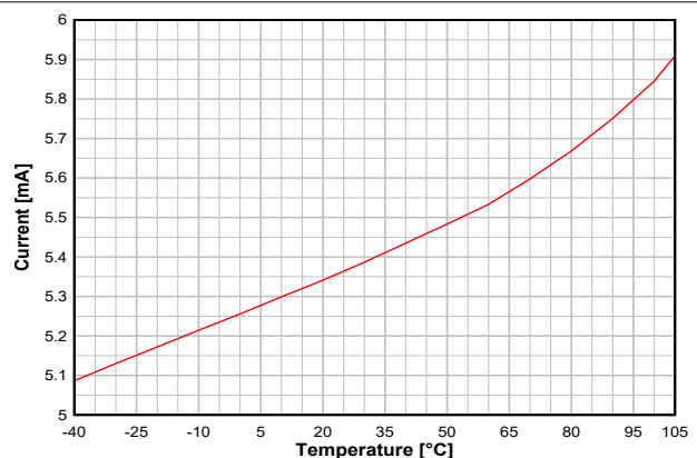
Figure 8-7. RX Current vs. Temperature (50 kbps, 868.3 MHz, VDD5 = 3.6 V)
