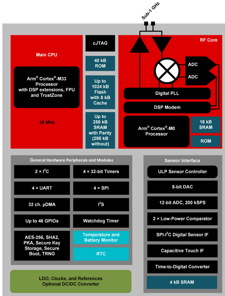
Figure 4-1. CC1314R10 Block Diagram
