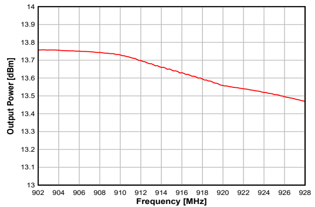
Figure 8-21. Output Power vs. Frequency (50 kbps, 915 MHz)
