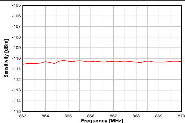
Figure 8-11. Sensitivity vs. Frequency (50 kbps, 868 MHz)
