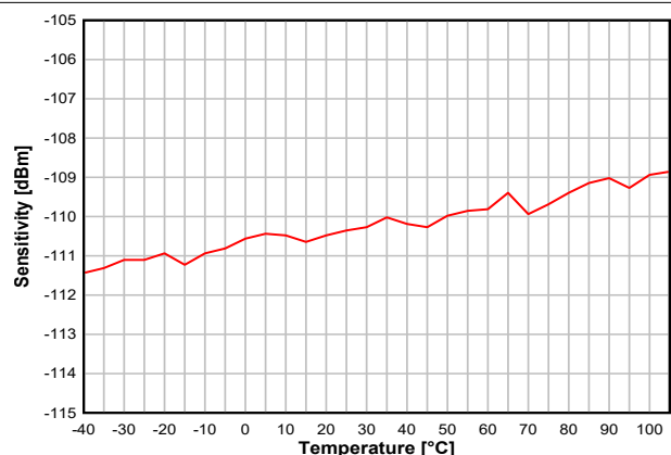
Figure 8-13. Sensitivity vs. Temperature (50 kbps, 868.3 MHz)
