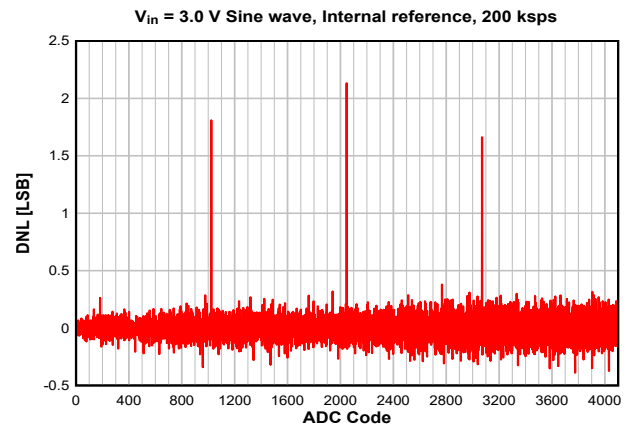
Figure 8-25. DNL vs. ADC Code
