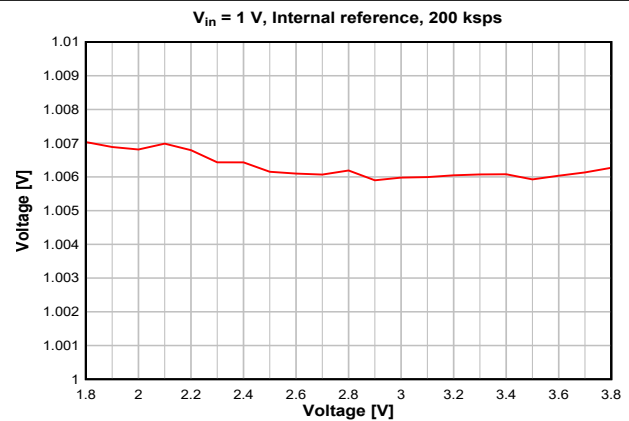
Figure 8-27. ADC Accuracy vs. Supply Voltage (VDD)
