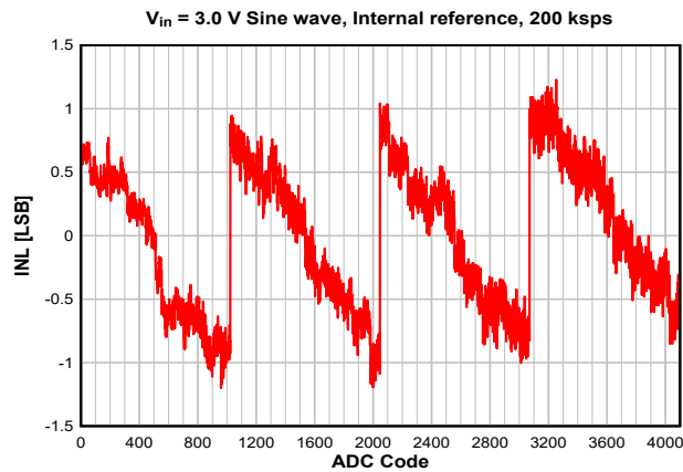
Figure 8-24. INL vs. ADC Code
