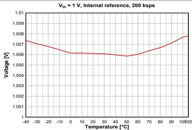
Figure 8-26. ADC Accuracy vs. Temperature
