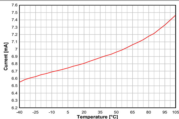
Figure 8-6. RX Current vs. Temperature (50 kbps, 868.3 MHz)
