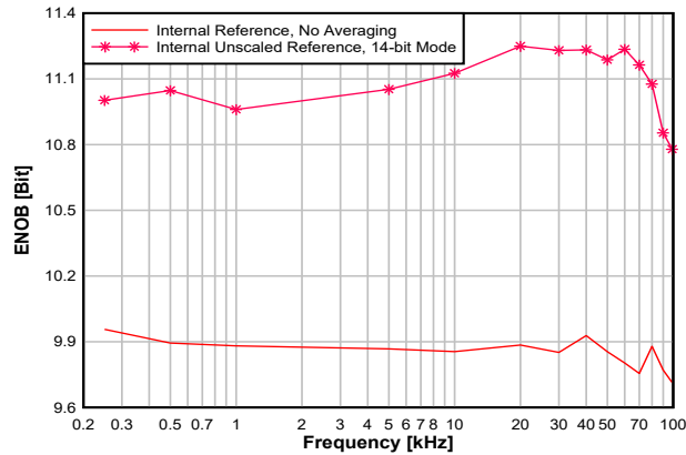
Figure 8-22. ENOB vs. Input Frequency
