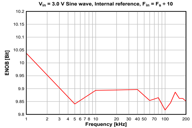
Figure 8-23. ENOB vs. Sampling Frequency
