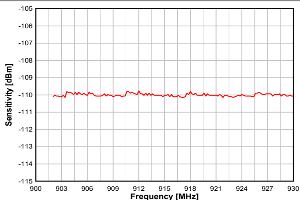
Figure 8-12. Sensitivity vs. Frequency (50 kbps, 915 MHz)
