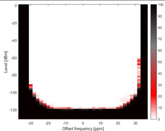
Figure 8-16. PER vs. Level vs. Frequency (SimpleLink™ Long Range 5 kbps, 868 MHz)
