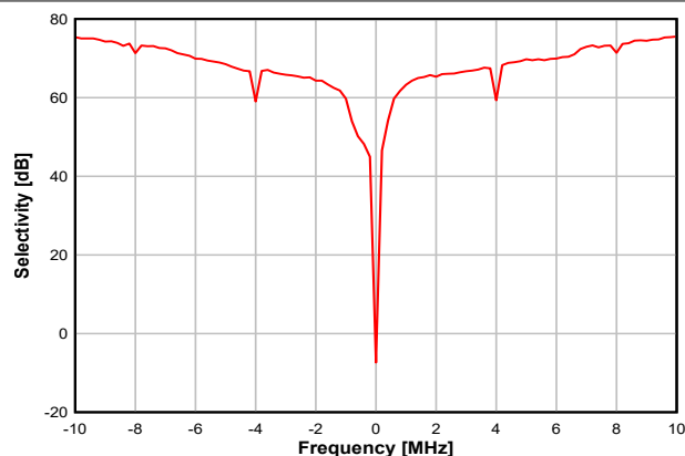
Figure 8-15. Selectivity vs. Frequency Offset (50 kbps, 868.3 MHz)
