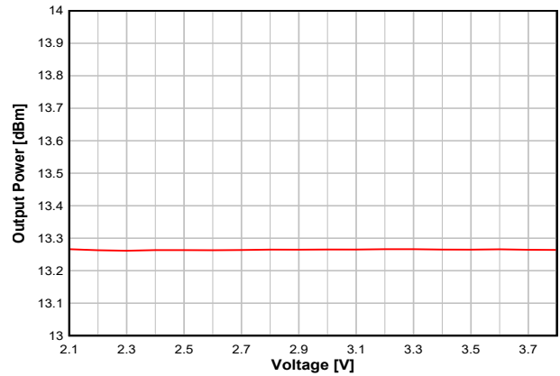
Figure 8-19. Output Power vs. Supply Voltage (VDD) (50 kbps, 868.3 MHz)
