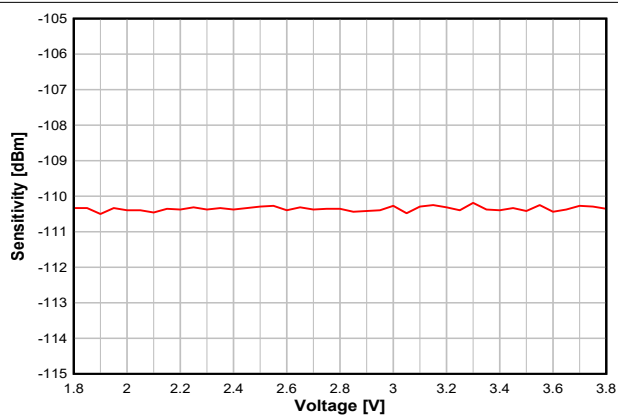
Figure 8-14. Sensitivity vs. Supply Voltage (VDD) (50 kbps, 868.3 MHz)
