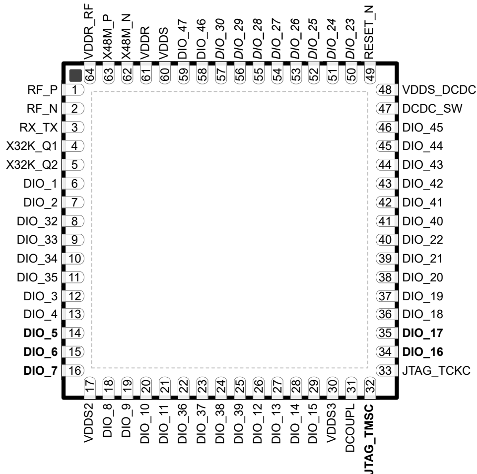
Figure 7-2. RSK (8 mm × 8 mm) Pinout, 0.4 mm Pitch (Top View)
