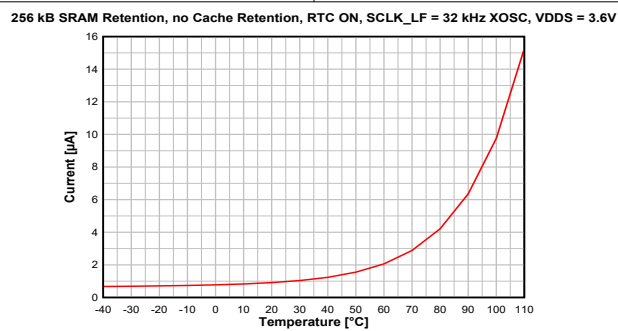
Figure 8-5. Standby Mode (MCU) Current vs. Temperature (VDD5 = 3.6 V)
