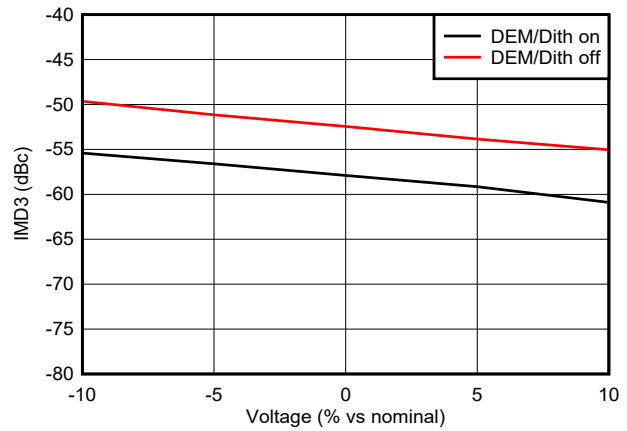
Figure 6-140. IMD3 vs Voltage in DES2XH Mode at 7247 MHz
