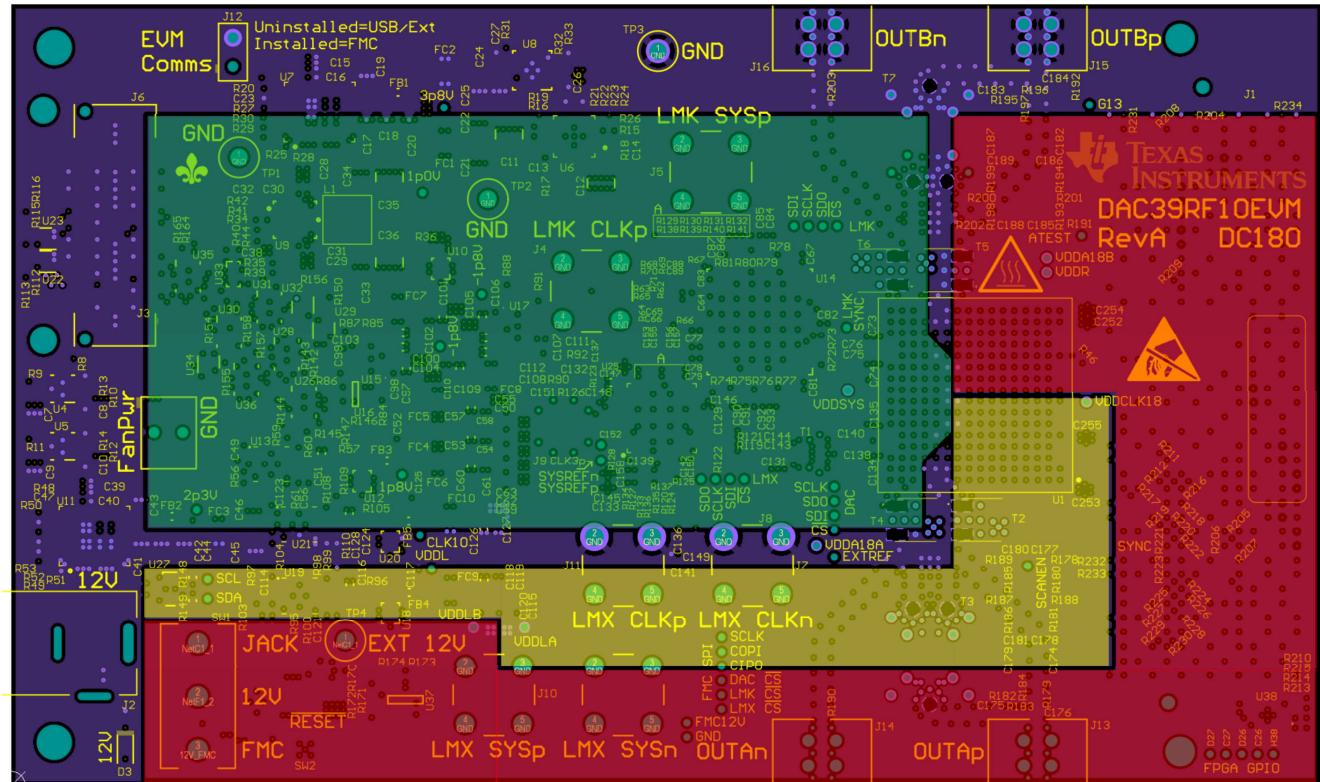
Layer5 / PWR2 DAC VDDL = RED DAC VDDLb = YELLOW DAC VDDCLK1P0V = GREEN Figure 8-32. Power Plane Layout for Layer 5
