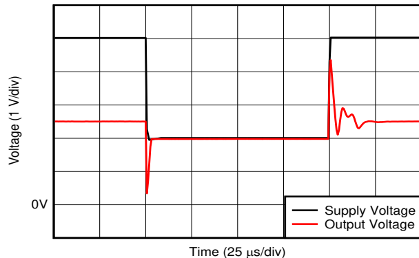
Figure 6-43. Supply Transient Response, A5 Devices
