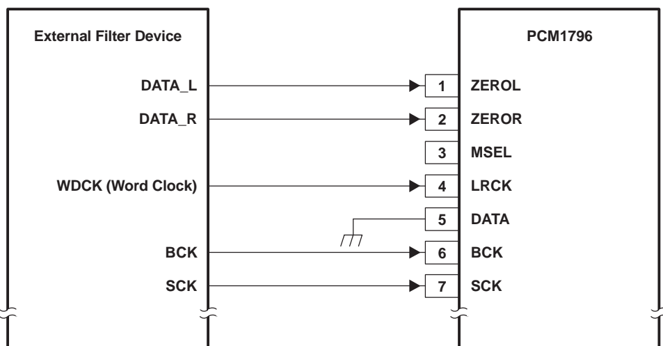
Figure 39. Connection Diagram for External Digital Filter (Internal DF Bypass Mode) Application
