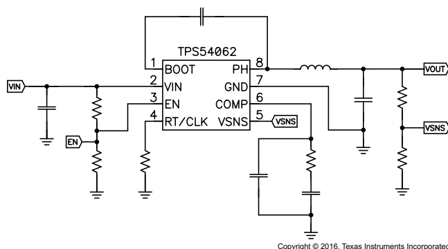
Simplified Schematic
