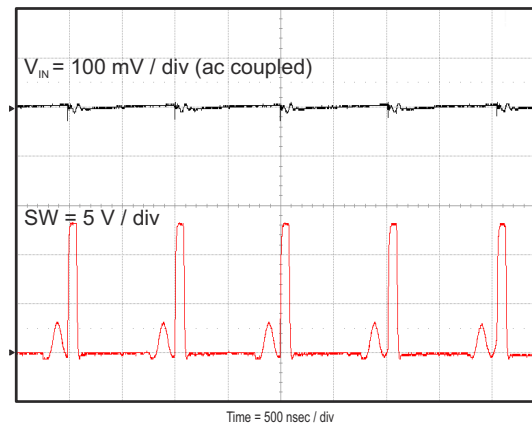
Figure 8-9. Input Voltage Ripple, I_{OUT} = 800 mA
