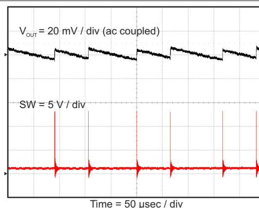
Figure 8-11. Output Voltage Ripple, I_{OUT} = 10 mA
