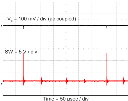
Figure 8-8. Input Voltage Ripple, I_{OUT} = 10 mA
