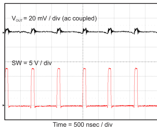
Figure 8-13. Output Voltage Ripple, I_{OUT} = 12 A
