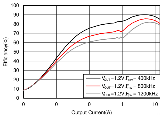
Figure 6-11. Efficiency with Internal VREG5 = 4.7 V, V_{IN} = 12\text{ V}
