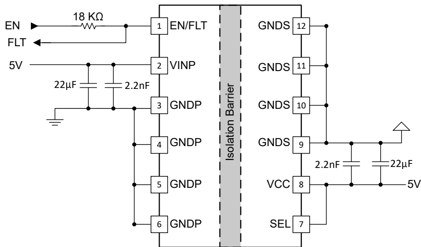
Figure 7-1. Typical Application
