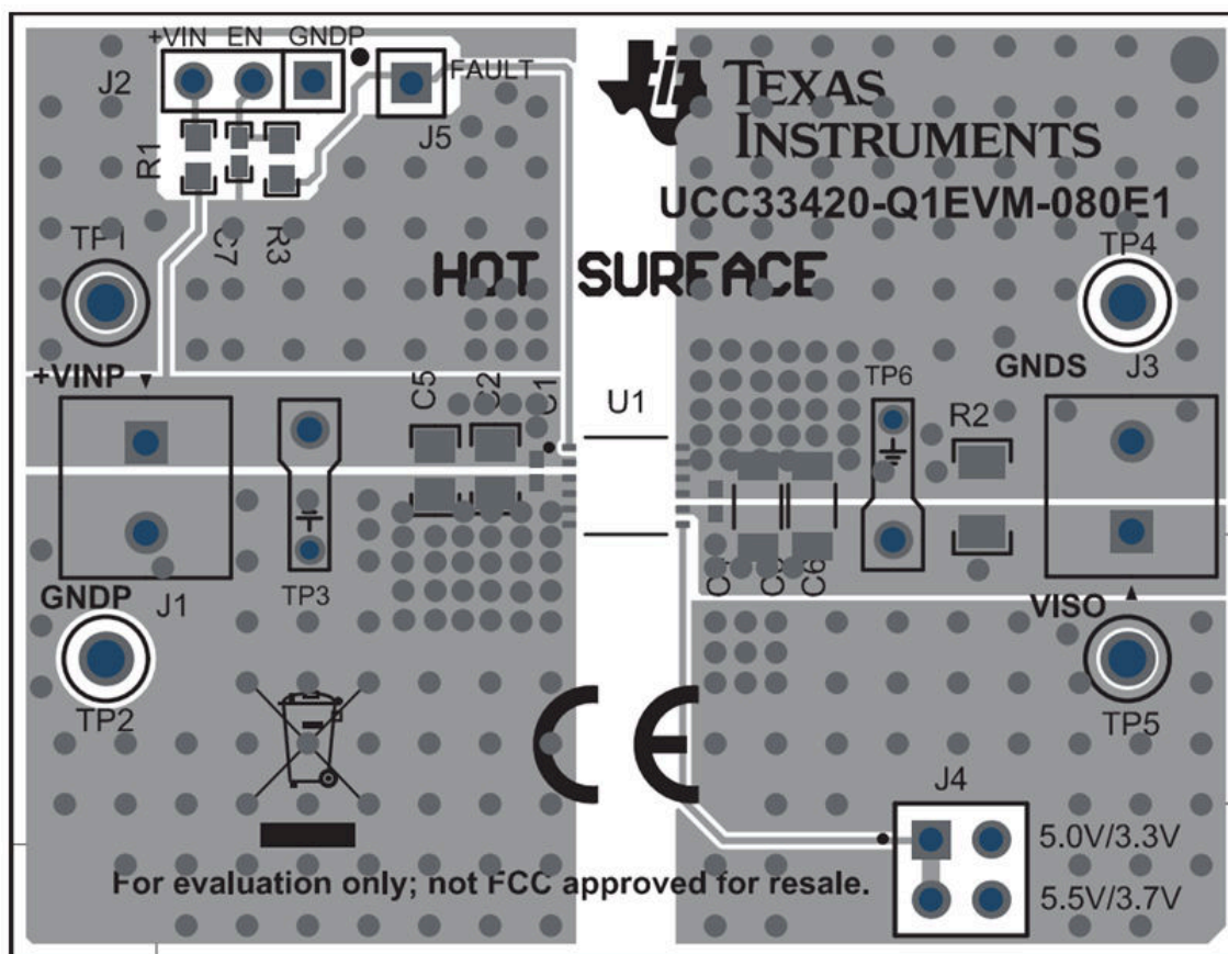
Figure 7-2. Layout Example
