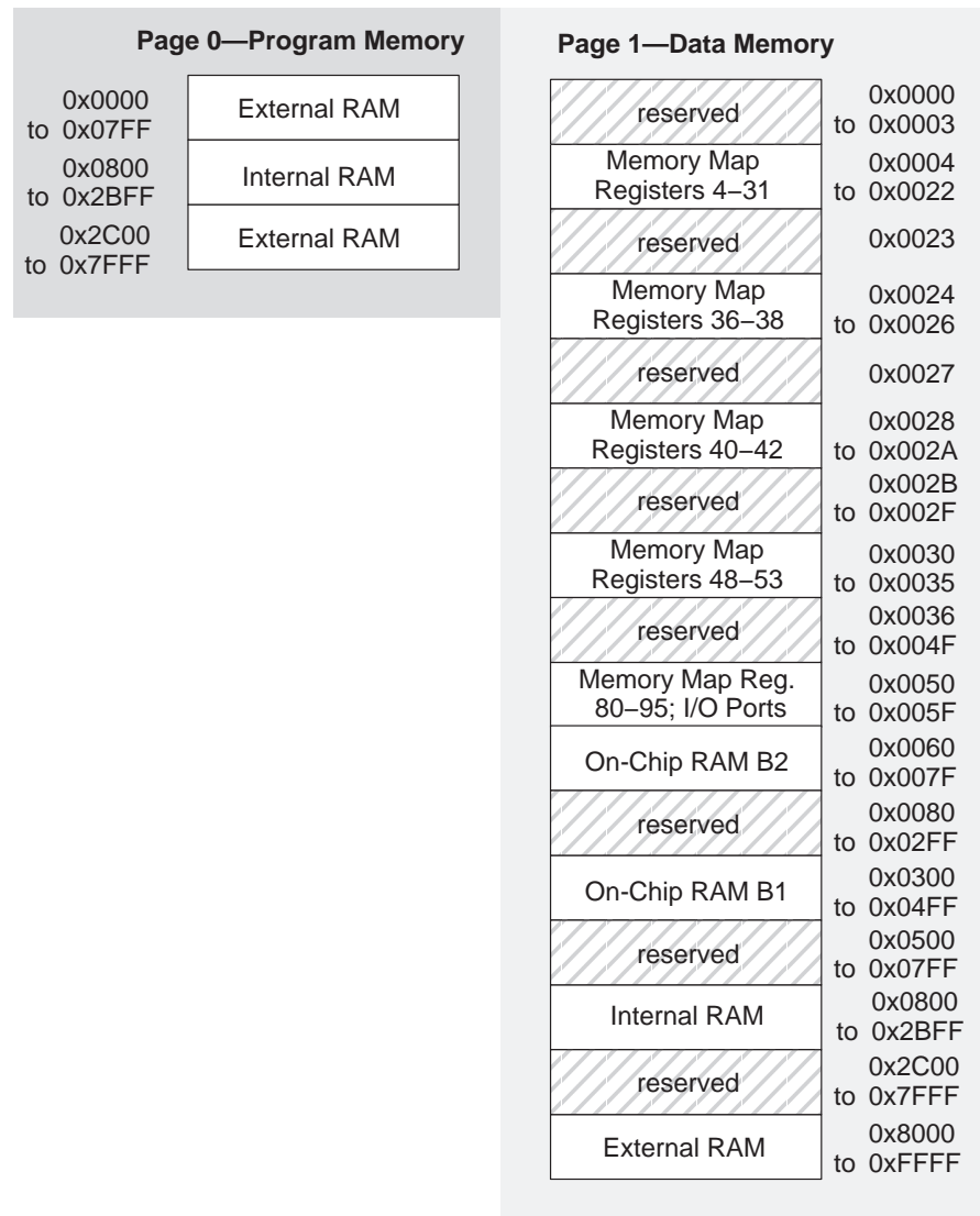
Figure 6–2. Sample Memory Map for Use With a 'C5x EVM
