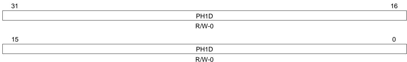
Figure 10. Pulse Width Modulator (PWM) First-Phase Duration Register (PH1D)
