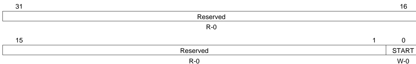
Figure 7. Pulse Width Modulator (PWM) Start Register (START)
