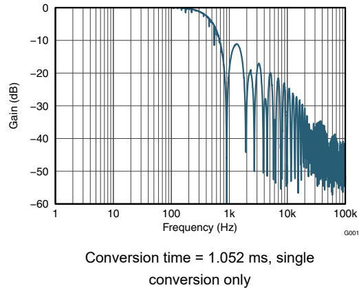
Figure 7-5. ADC Frequency Response
