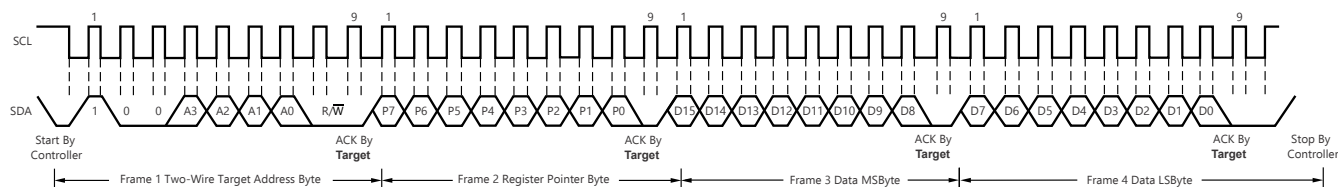
Figure 7-9. Timing Diagram for Write Word Format
