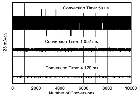
Figure 7-6. Noise vs Conversion Time (Averaging = 1)
