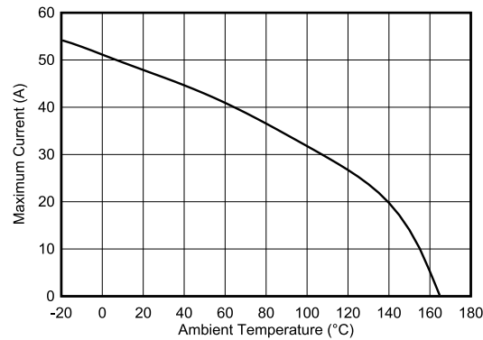
Figure 7-1. Maximum Continuous Shunt Current vs Ambient Temperature
