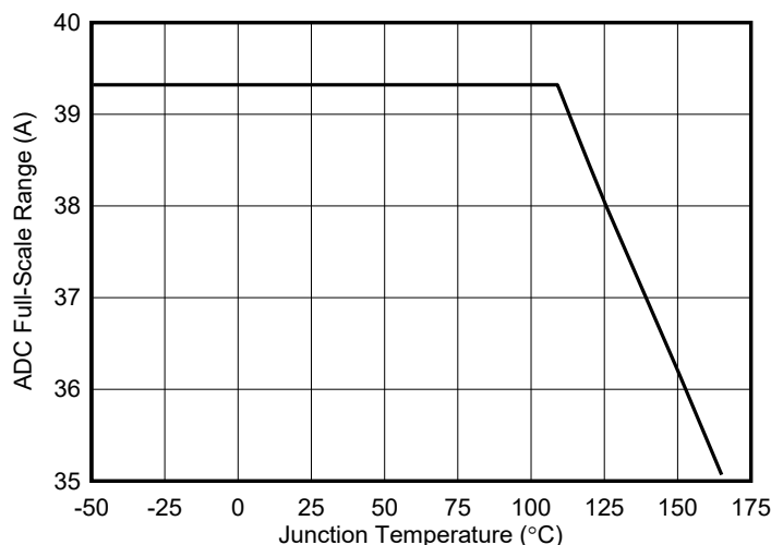
Figure 8-1. Maximum ADC Current Reading vs Junction Temperature
