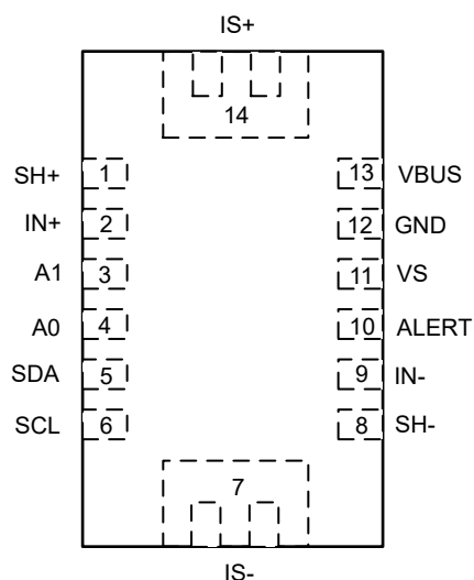
Figure 5-1. REL Package 14-Pin QFN Top View
