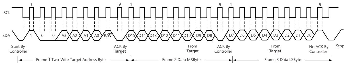
Figure 7-9. Timing Diagram for Write Word Format
