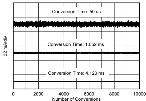
Figure 7-7. Noise vs Conversion Time (Averaging = 128)
