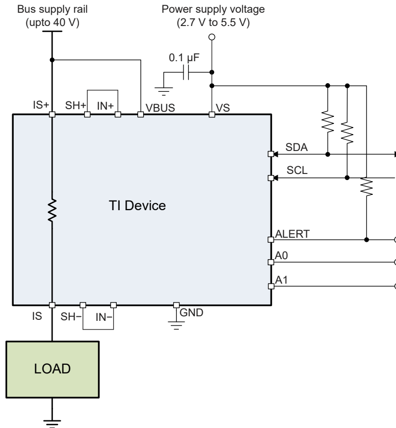
Figure 8-2. INA746 High-Side Sensing Application Diagram
