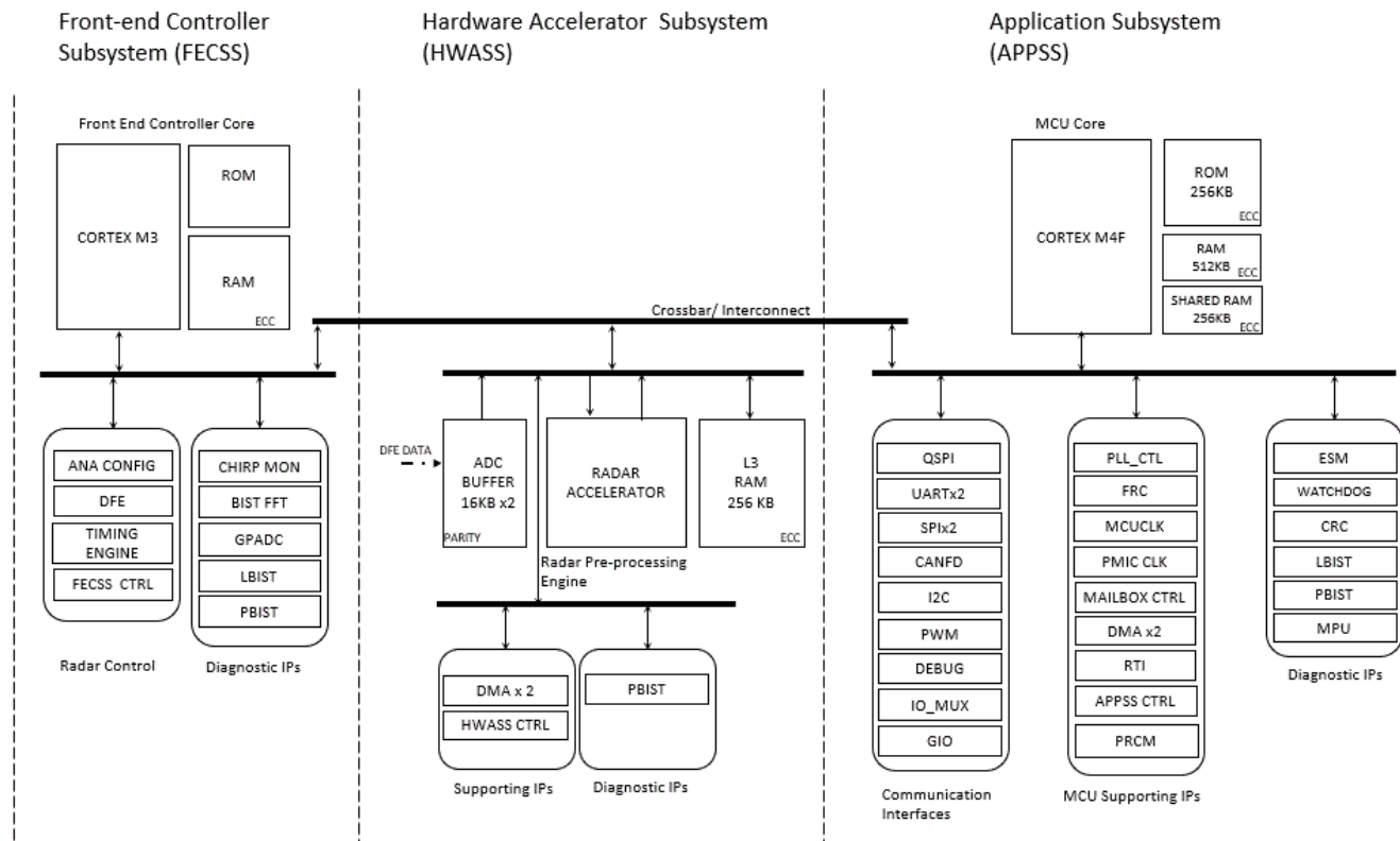
Figure 9-5. Processor Subsystem
