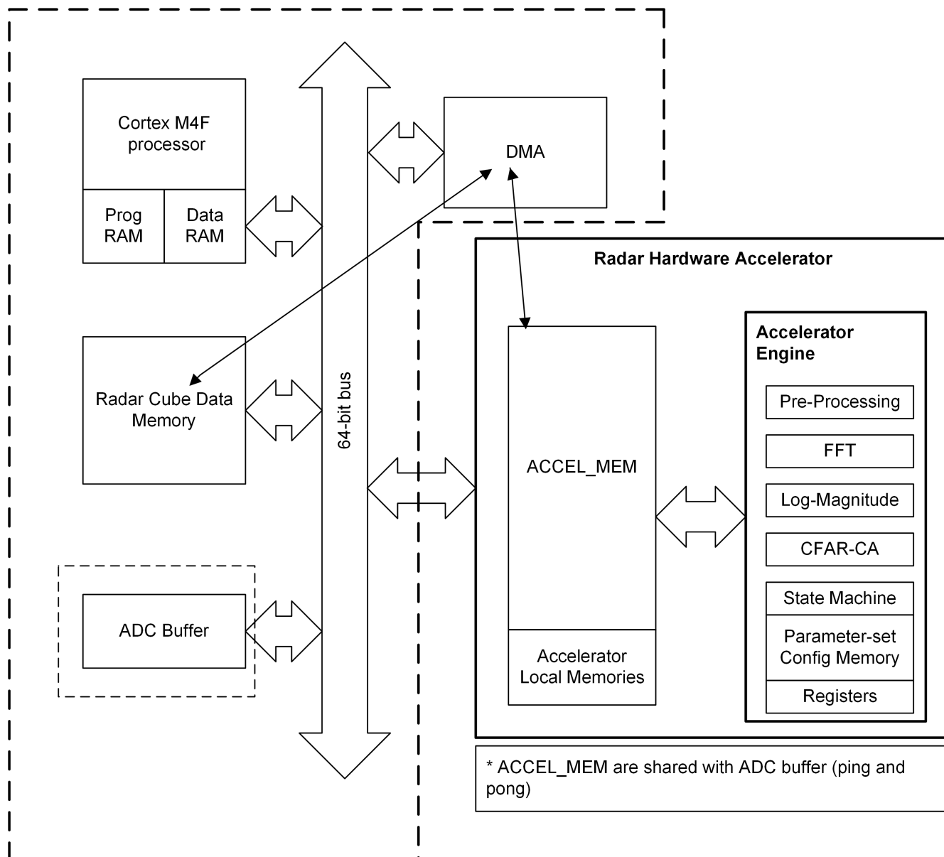
Figure 9-6. HWA 1.2 Functional Block Diagram
