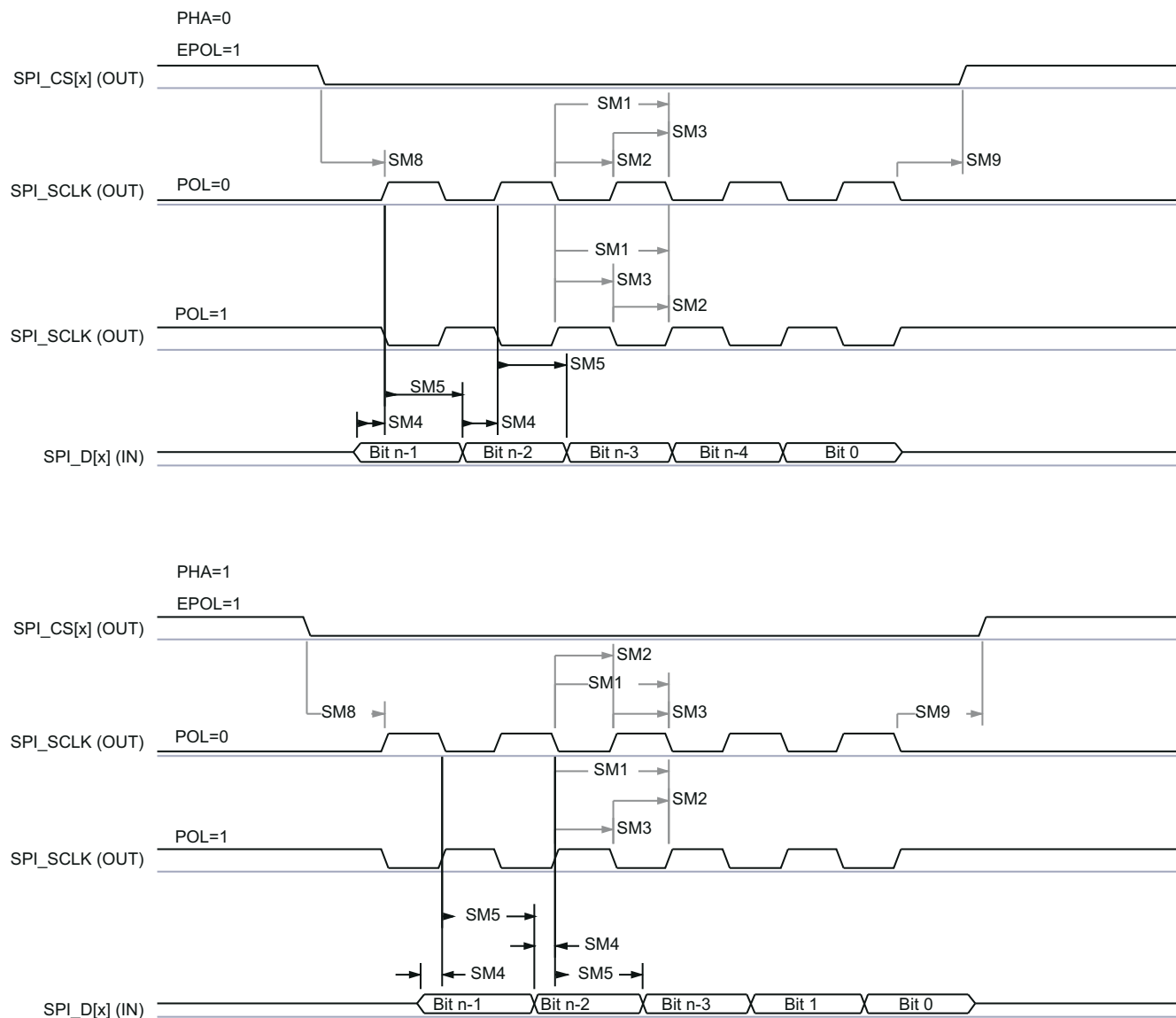
Figure 8-9. SPI Timing -Controller Mode Receive
