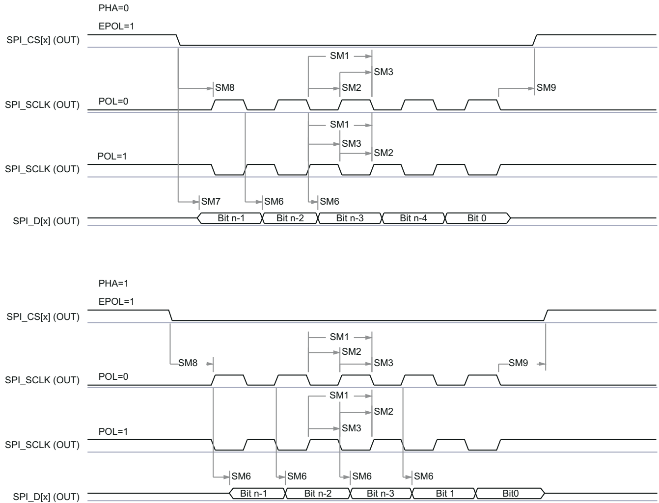
Figure 8-10. SPI Timing- Controller Mode Transmit
