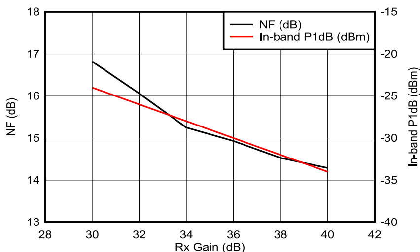
Figure 8-4. Noise Figure, In-band P1dB vs Receiver Gain
