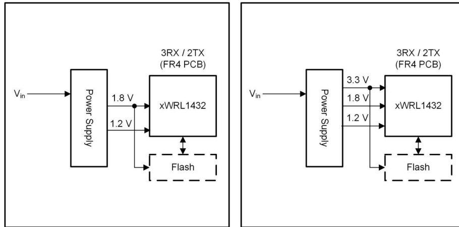
Figure 8-3. Power Optimized Mode Power Management (Left: 1.8V I/O Topology, Right: 3.3V I/O Topology)
