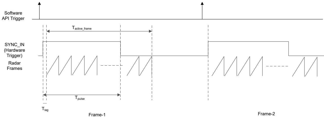
Figure 8-7. Sync In Hardware Trigger
