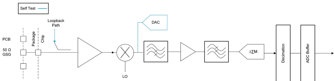
Figure 9-4. Receive Subsystem (Per Channel)
