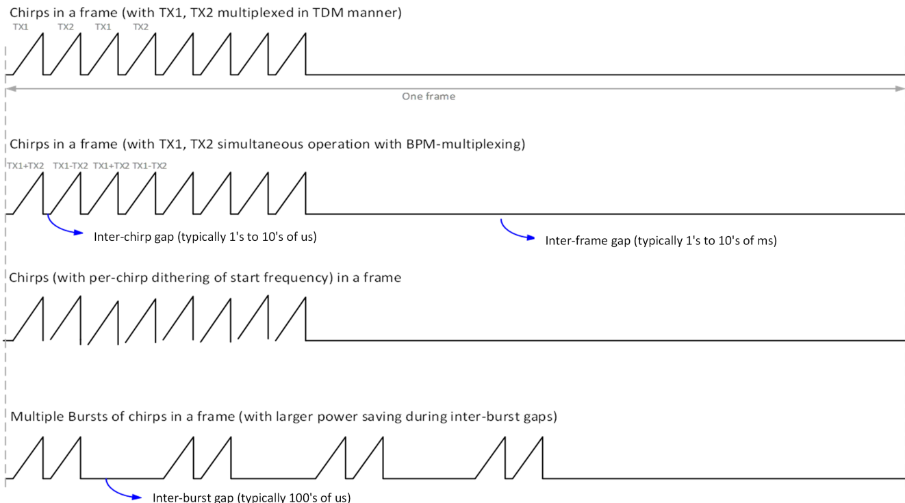
Figure 8-5. Chip Profile Supported by Timing Engine
