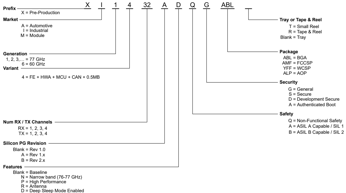
Figure 11-1. Device Nomenclature
