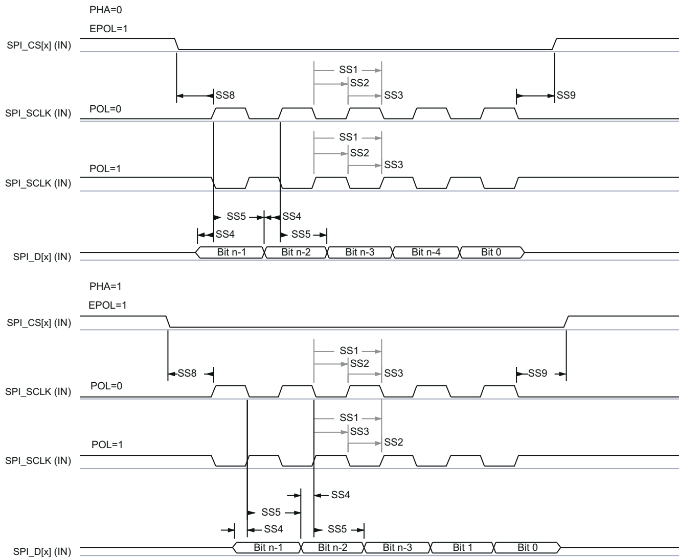
Figure 8-11. SPI Timing - Peripheral mode Receive
