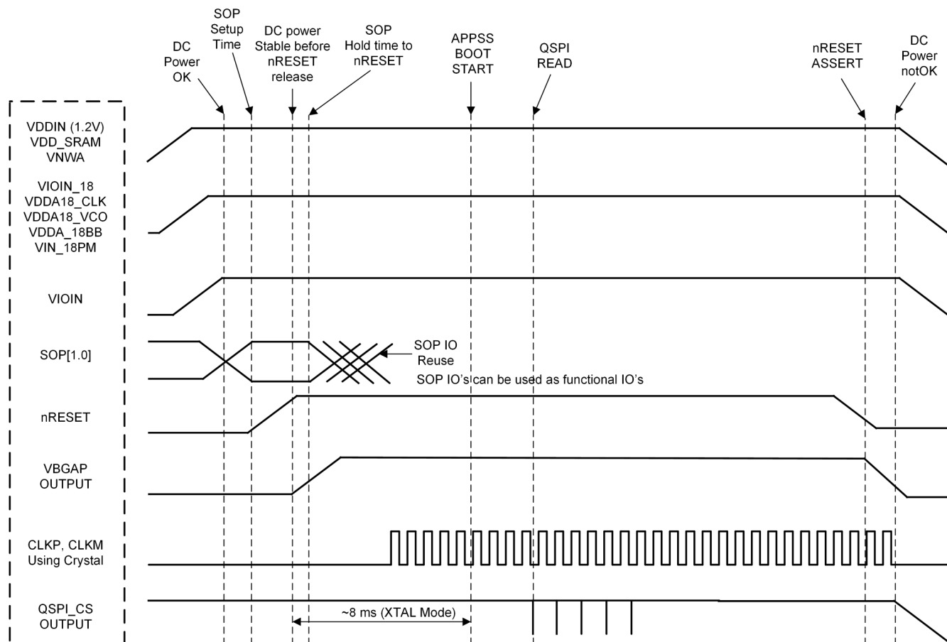
Figure 8-6. Device Wake-up Sequence
