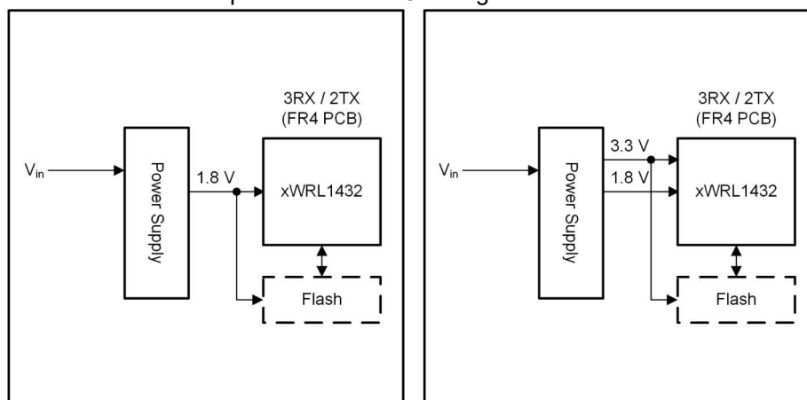
Figure 8-2. BOM Optimized Mode Power Management (Left: 1.8V I/O Topology, Right: 3.3V I/O Topology)
