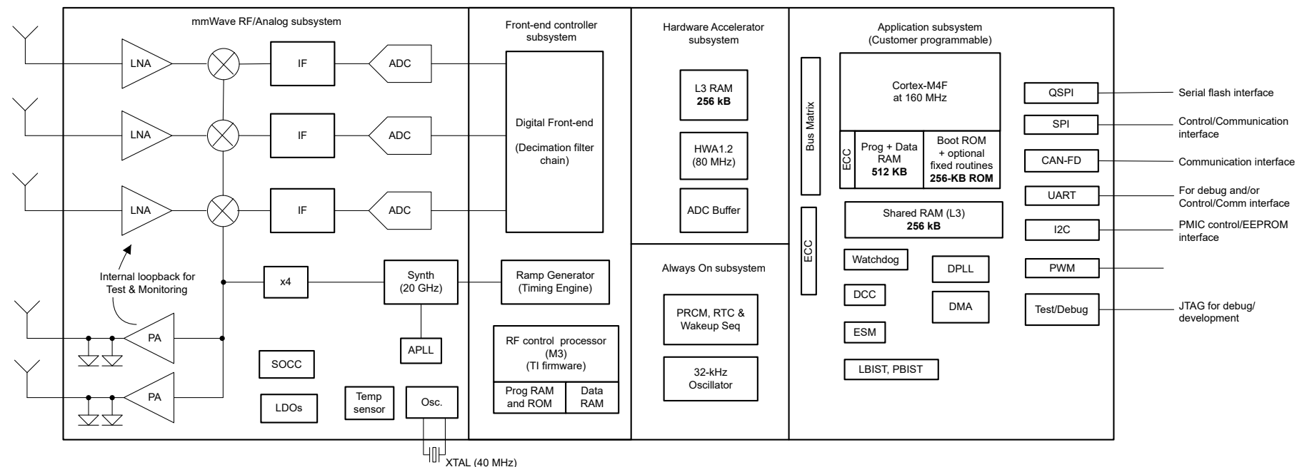
Figure 9-1. Functional Block Diagram
