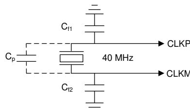
Figure 8-8. Crystal Implementation
