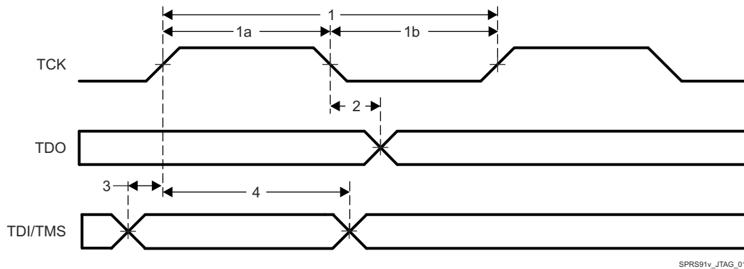
Figure 8-18. JTAG Timing
