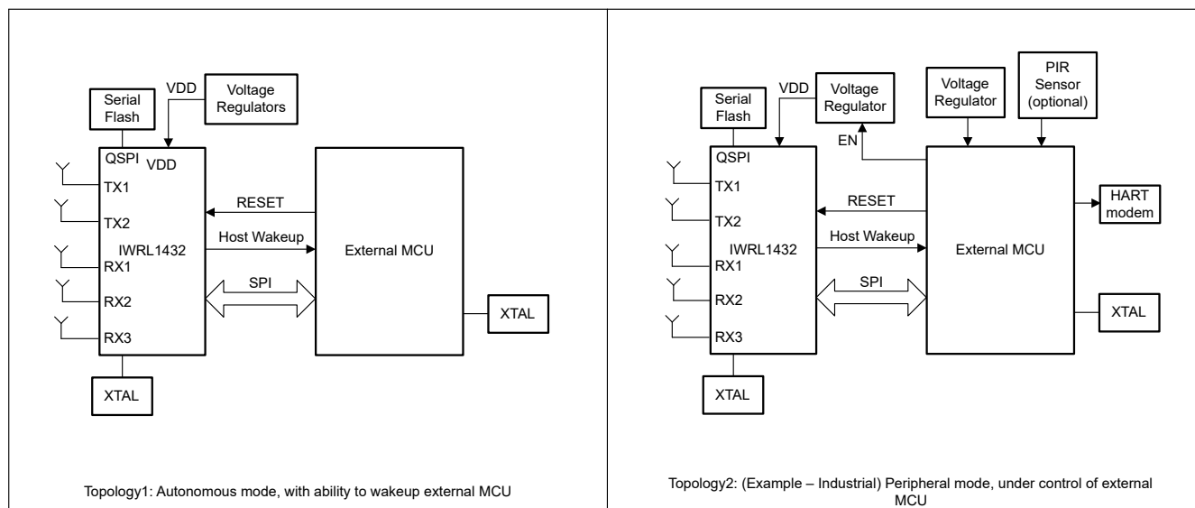
Figure 8-1. System Topologies
