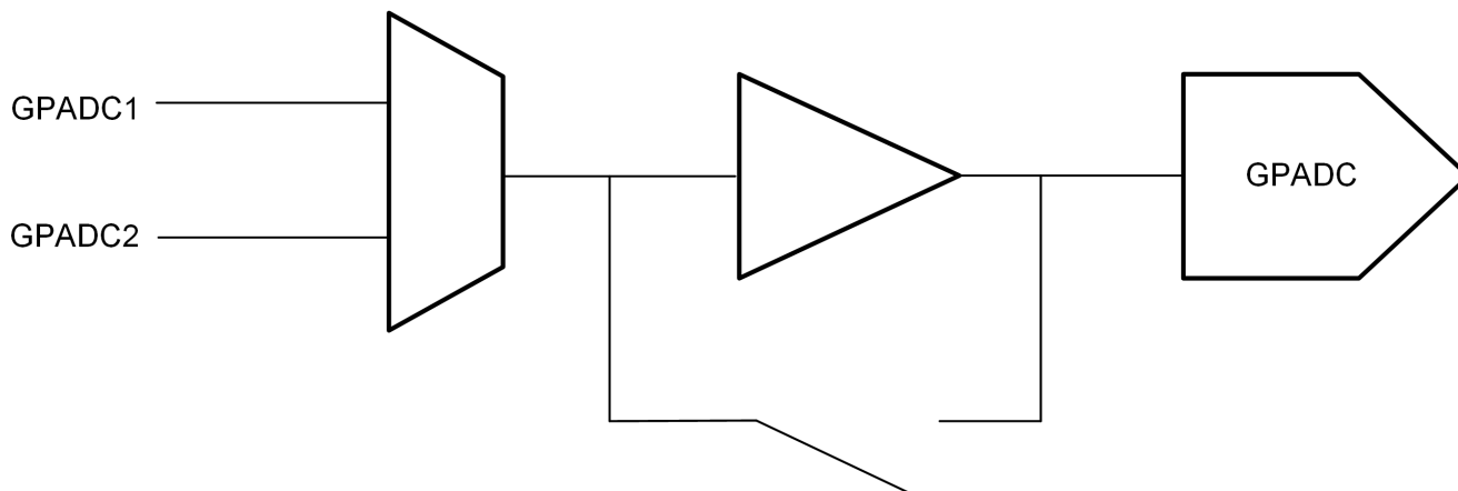
Figure 9-7. GPADC Path
