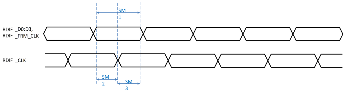
Figure 8-13. RDIF Timing Requirements
