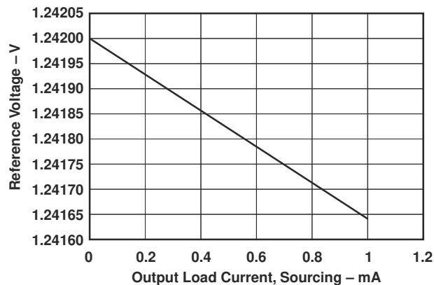
Figure 7-16. Reference Voltage vs Output Load Current (Sourcing)
