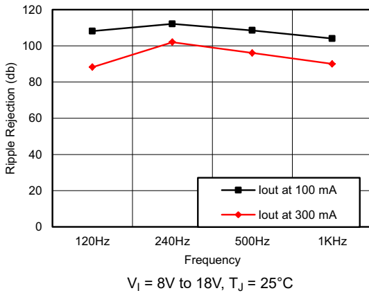
Figure 5-9. PSRR vs Frequency and I_O (Legacy Chip)
