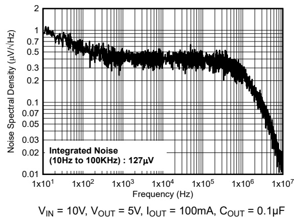
Figure 5-11. Noise vs Frequency (New Chip)
